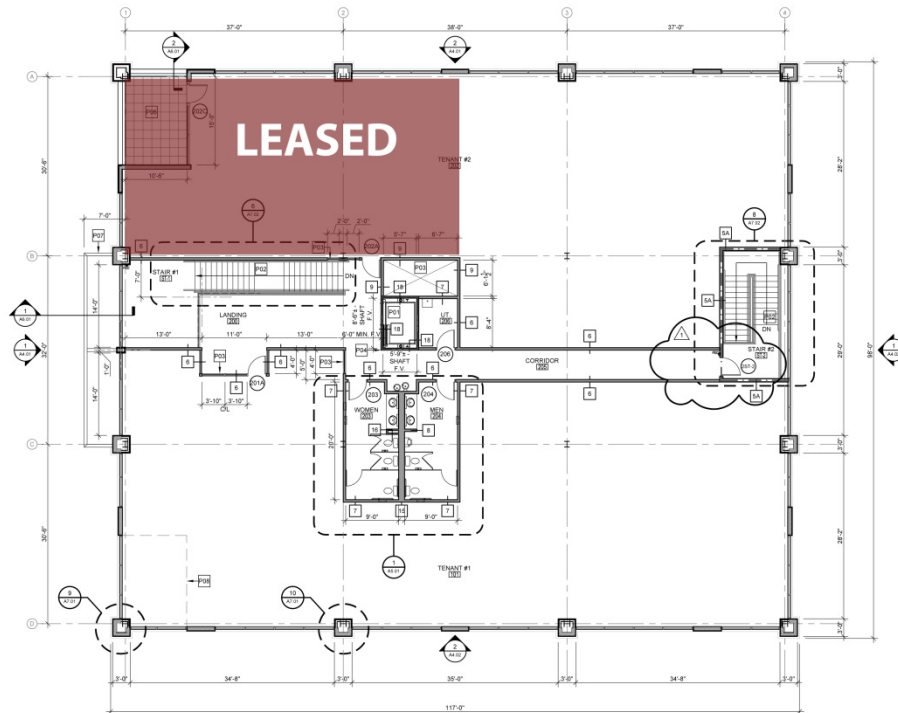
1 Partition Plan @ SECOND FLOOR A2.02 SCALE 1/8" = 1'-0"
