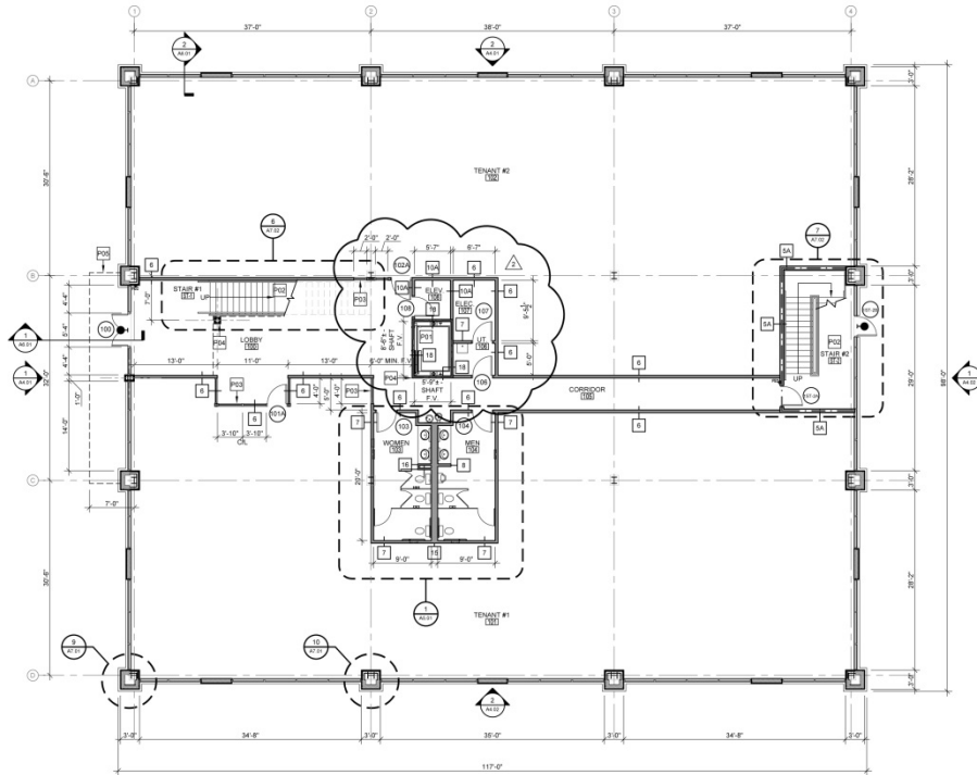
1 Partition Plan @ FIRST FLOOR A2.01 SCALE 1/8" = 1'-0"
